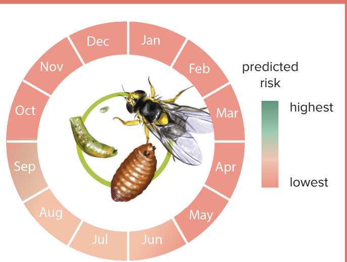
Average predicted seasonality of VLM within 100km of Carnarvon, WA.
