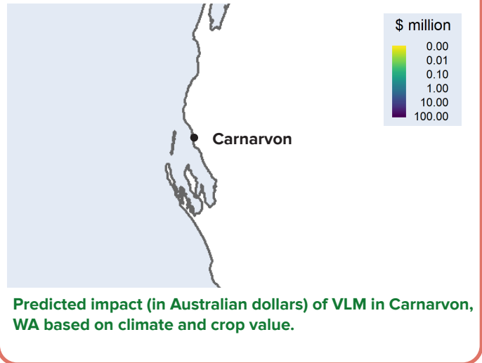
Fig 1. Predicted impact in Carnarvon
